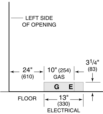
Electrical Location Illustration
