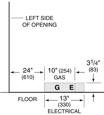
Gas Supply Illustration
