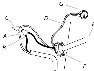
A. White wires B. Black wires C. UL listed wire connector D. Green (or bare) ground wire E. Homepower supply cable F. UL listed or CSA approved 1/2" strain relief G. Green ground screw
