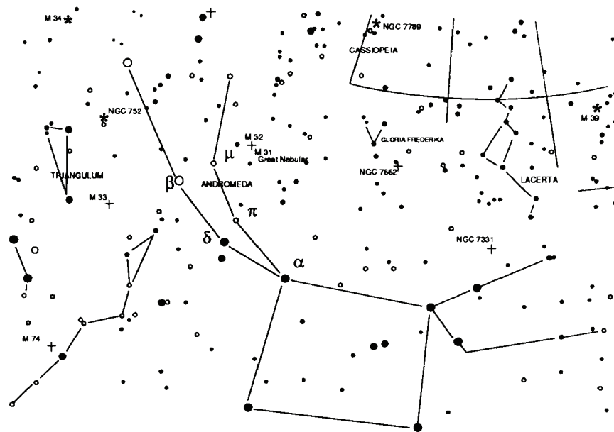
Fig. 16 Galassia Andromeda
