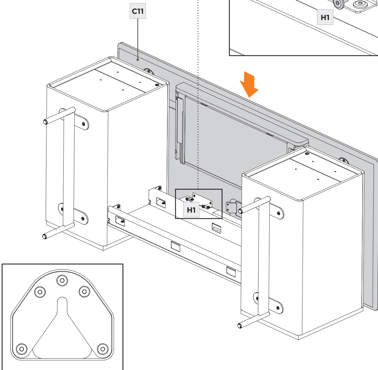
Detail of Connection Plate
